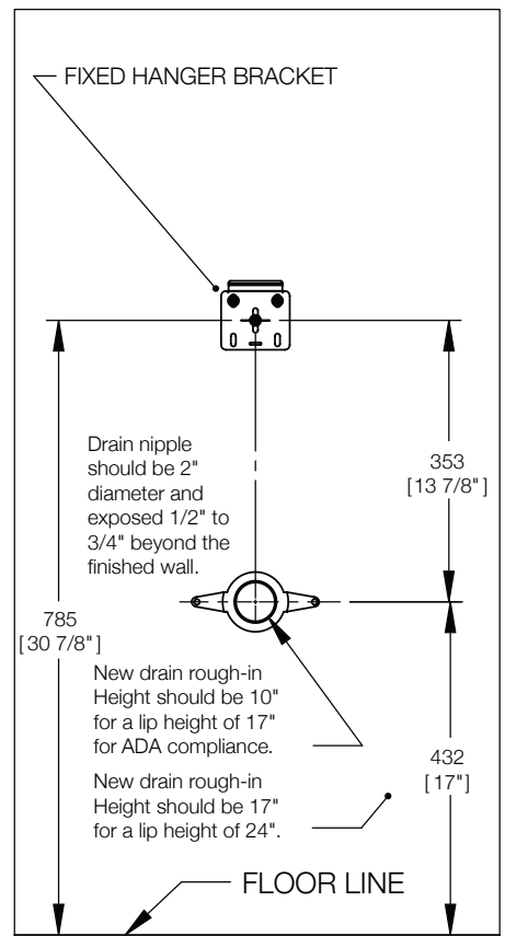
Rough-in & Bracket Location
